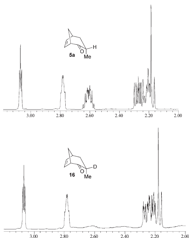
Figure 1. ^1\text{H} NMR spectra (2.0–3.2 ppm) of 5a and 16 .
